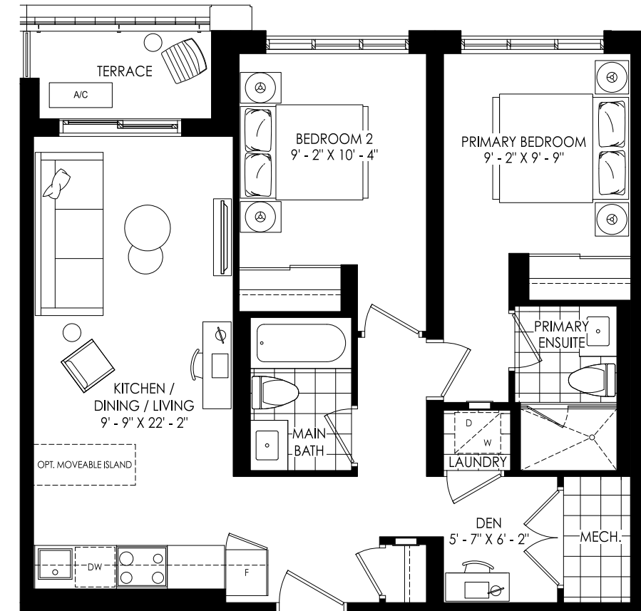
THIRD FLOOR
