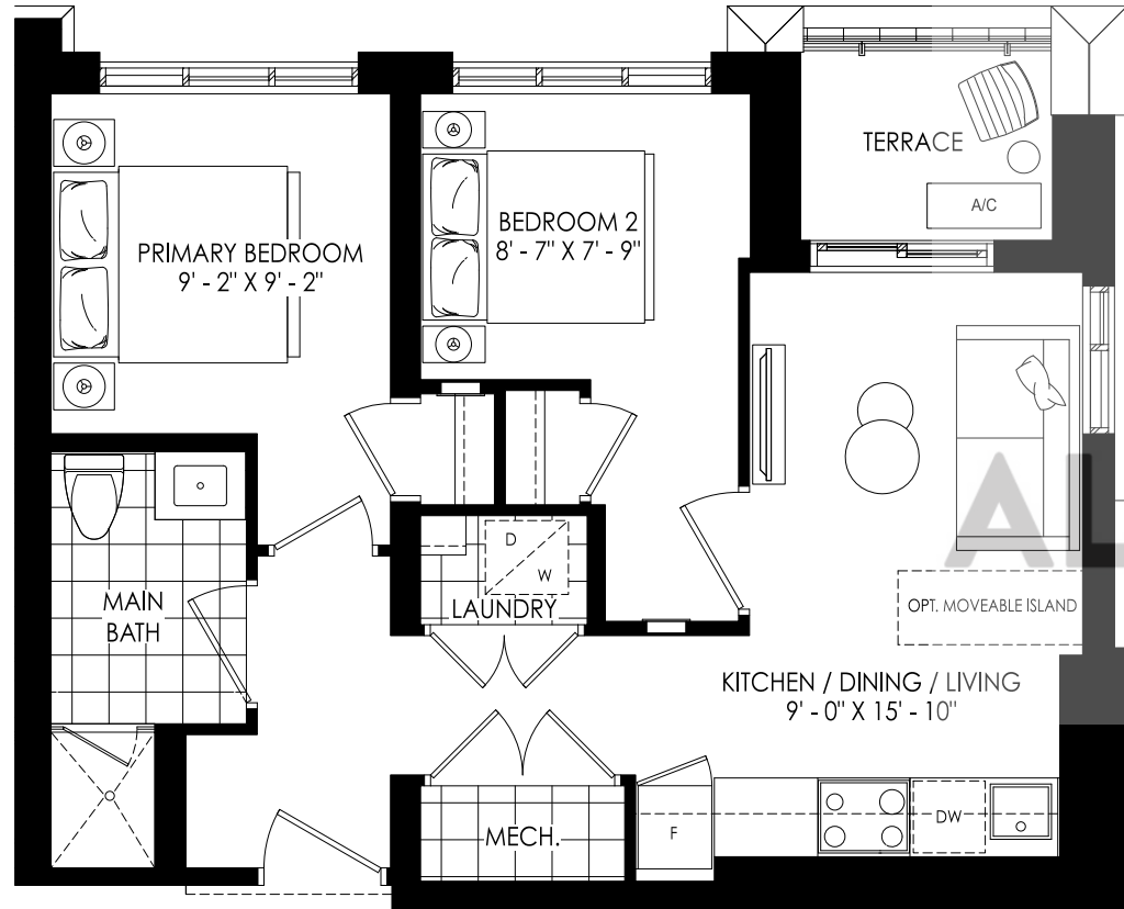
THIRD FLOOR
