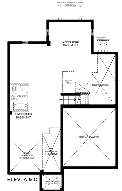
LOWER LEVEL
