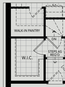
PARTIAL OPT. MAIN LEVEL FOR UPPER LEVEL LAUNDRY
