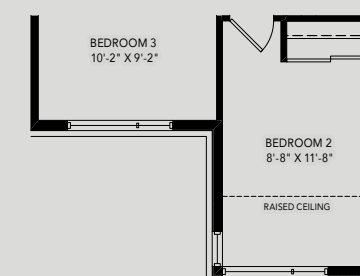
PARTIAL UPPER LEVEL
