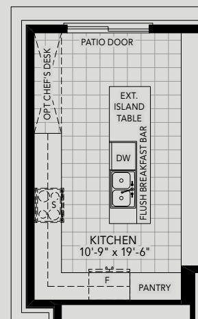
PARTIAL OPT. KITCHEN MAIN LEVEL
